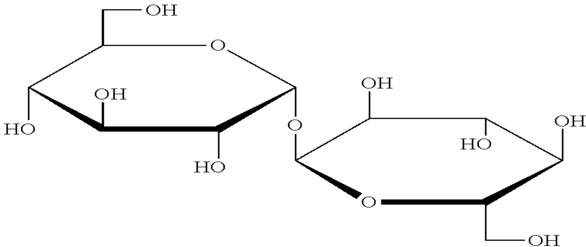
α D-glucopyranosyl (1→1) α D-glucopyranoside.
