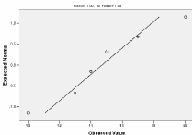
Normal Q-Q Plot of Data
