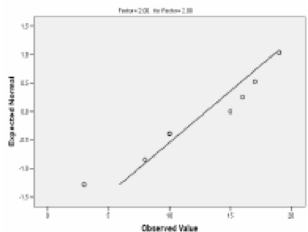
Normal Q-Q Plot of Data
