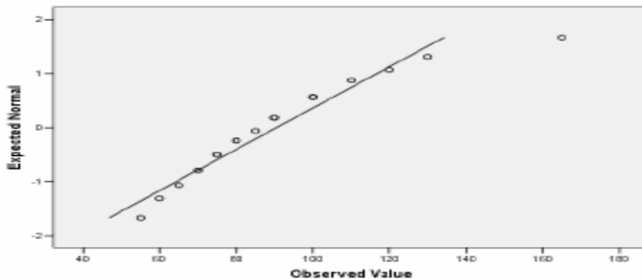
Normal Q-Q Plot of weight
