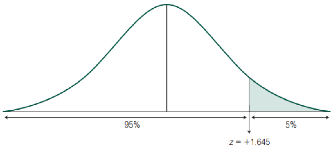
B. Curve showing the critical region for a directional test (one-tailed test)
