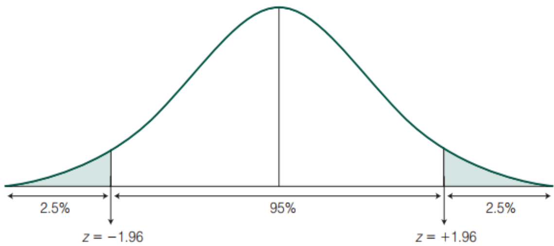
A. Curve showing the critical region for a nondirectional test (two-tailed test)
