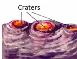
Hawaiian-type
